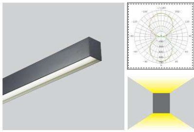
S-吊装 S-suspended
